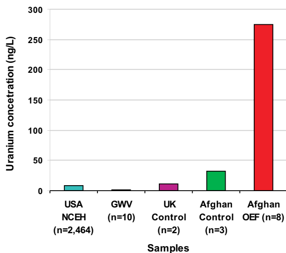
Figure 4. Concentration of uranium isotopes in the 24-hour-urine samples of symptomatic civilians and controls after the bombing raids in the Operation Enduring Freedom (OEF), Afghanistan, 2002. NCEH – National Committee of Environmental Health; GWV – Gulf War veterans.
